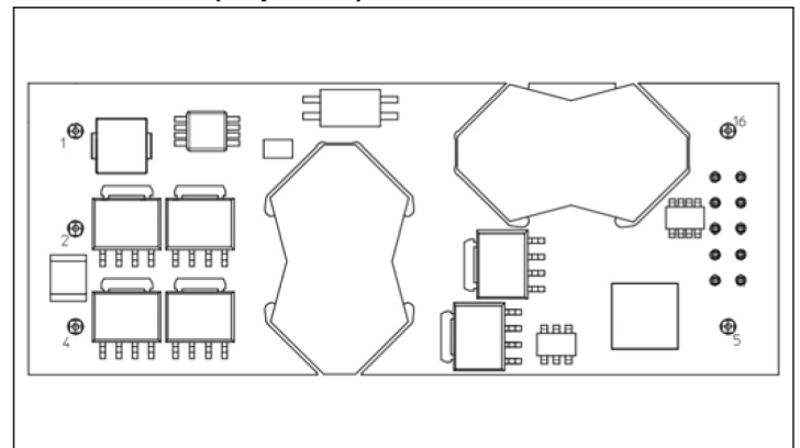
(Best air flow direction is from negative to positive pins.)
